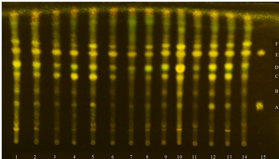
1-14. 红牛膝药材(8号作为红牛膝对照药材); 15. 对照品(A. 人参皂苷 R_0 ; E. \beta -蜕皮甾酮); A-F. 特征荧光斑点。 1-14. Hongniuxi medicinal materials (No. 8 is the reference material of Hongniuxi); 15. Reference substance (A. Ginsenoside R_0 ; E. \beta -ecdysterone); A-F. Characteristic fluorescent spots.
